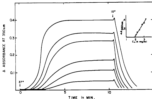
FIGURE 1: Effect of c-tubulin concentration on development of turbidity in the presence of 5 \times 10^{-6} M nocodazole. The solvent was 10^{-2} M Mes, 5 \times 10^{-4} M GTP, 1.0 \times 10^{-3} M \text{MgCl}_2 , 2 \times 10^{-3} M EGTA, and 1% (v/v) \text{Me}_2\text{SO} at pH 6.9.
